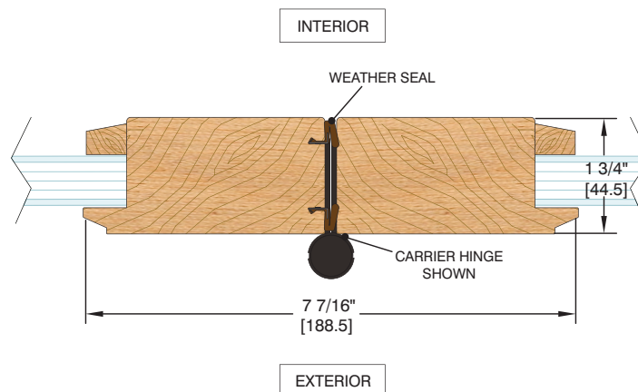
MEETING PANEL PLAN VIEW
