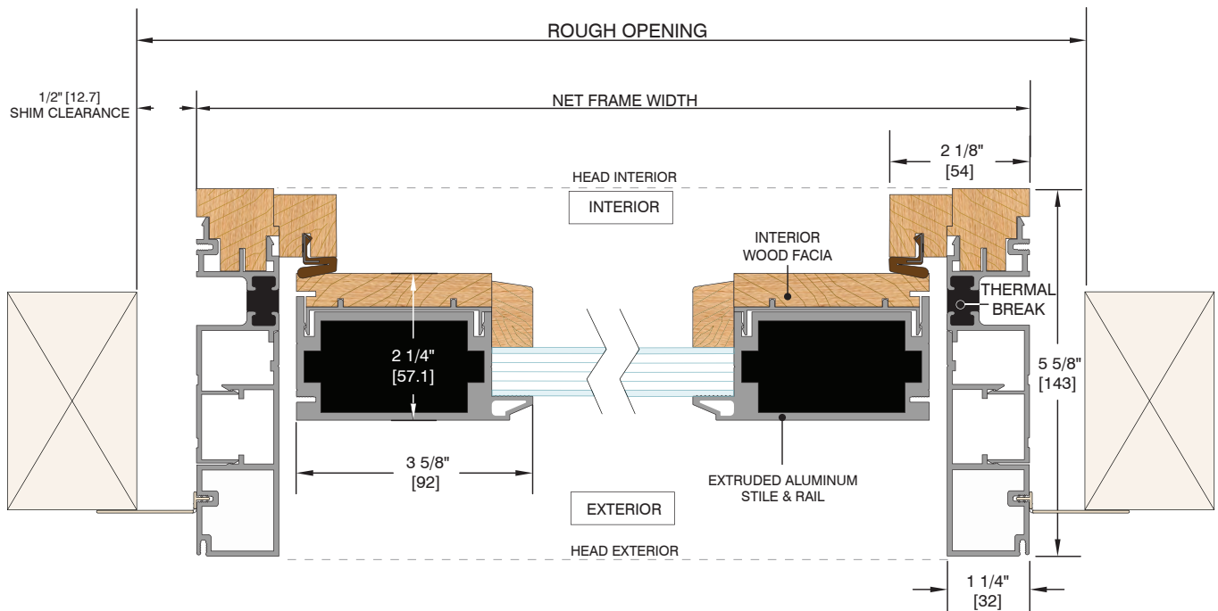
JAMB PLAN VIEW
