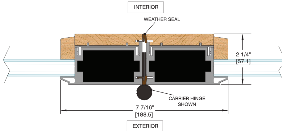
MEETING PANEL PLAN VIEW
